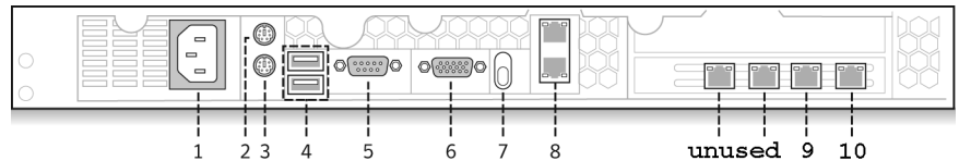
Figure 37-2 Enforcer appliance back panel (Failopen model shown)
